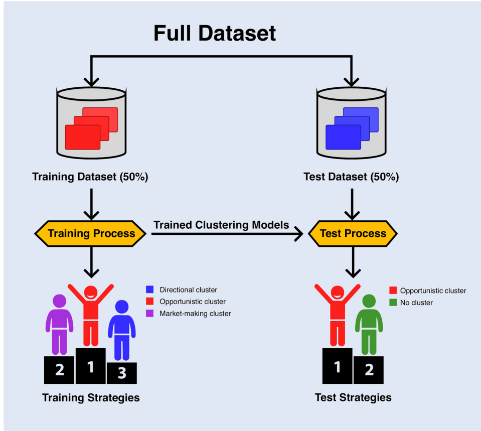
Figure 3. Schematic diagram of the ClusterLOB: We identify the best trading strategy with the highest SR in the training dataset, and demonstrate that its performance outperforms benchmark trading strategies that do not incorporate clustering in the test dataset.
